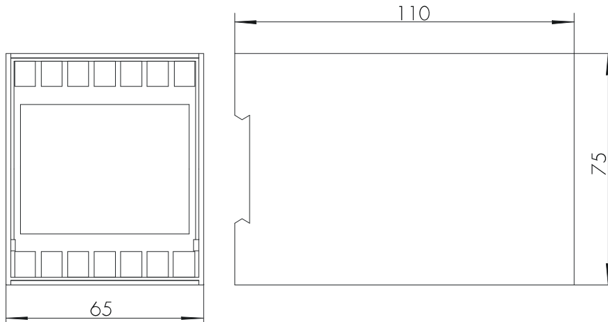
Figure 5.1: Dimensional drawing
