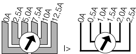
Figure 4.3: Adjustment example
